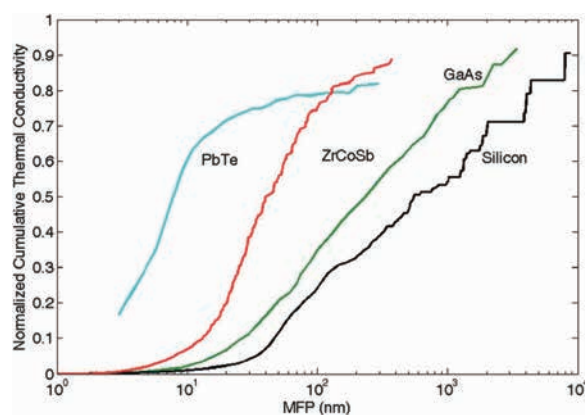
Fig 2. Accumulated thermal conductivity versus the mean free path for the same materials as in Fig 1. at T=300K
