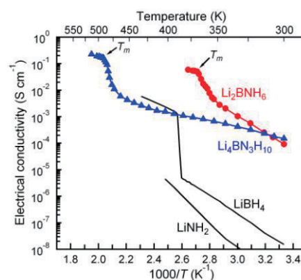
Fig. 2 Electrical conductivities of \text{Li}_2\text{BNH}_6 and \text{Li}_4\text{BN}_3\text{H}_{10} . The melting temperatures are indicated as T_m . For reference, the data of the host hydrides \text{LiBH}_4 and \text{LiNH}_2 are also shown.
