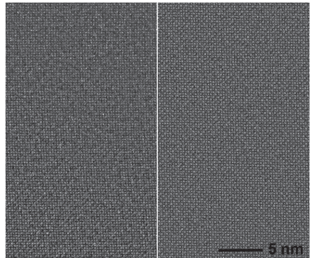
Fig. 2 HAADF-STEM images of two regions of similar thicknesses (as attested by low-loss EELS spectra) from a 1.4 at. % Yb-doped sample (left) and a pure YAG sample (right).
