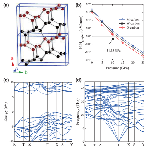
Fig. 1 The orthorhombic O-carbon in Pbam symmetry. (a) A polyhedral view of the crystal structure. (b) The enthalpy per atom (relative to that of graphite) for M-carbon, W-carbon, and O-carbon versus pressure. (c) Calculated electronic band structure of O-carbon at 15 GPa; (d) Calculated phonon dispersion curves of O-carbon at 15 GPa.
