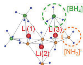
Fig. 1 Local atomic structure of the complex hydride \text{Li}_4\text{BN}_3\text{H}_{10} . \text{Li}_4(\text{BH}_4)(\text{NH}_2)_3 have plural occupation sites for \text{Li}^+ ions with different tetrahedral coordination consisting of [\text{BH}_4]^- and [\text{NH}_2]^- anions
